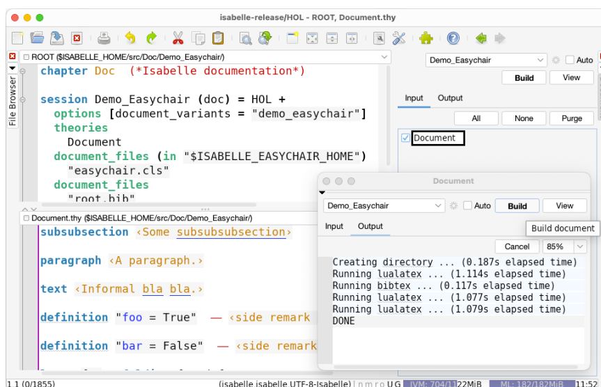
Figure 4.5: Document panel with separate instances for Input and Output
